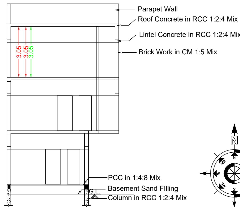
Section RR
