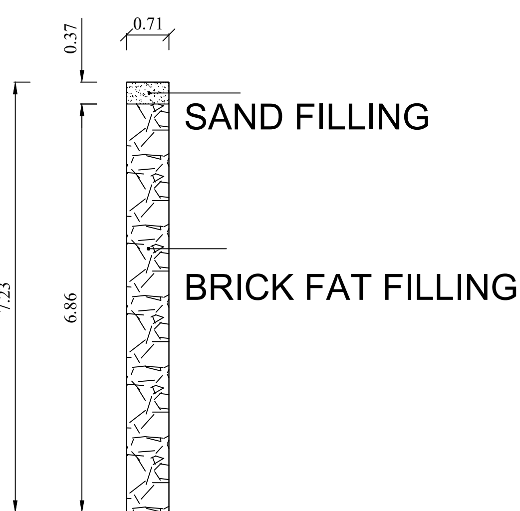
DETAILS OF PERCULATION PIT
