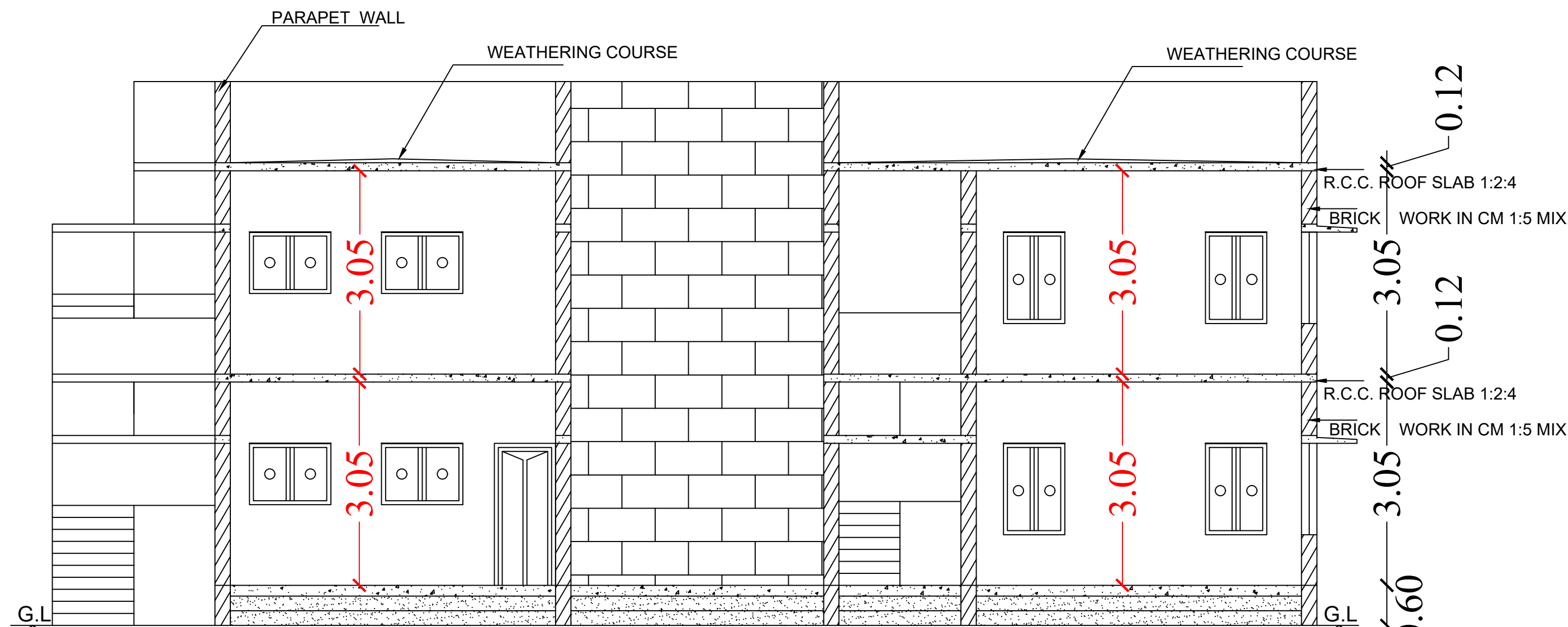
Section on-"AA"
