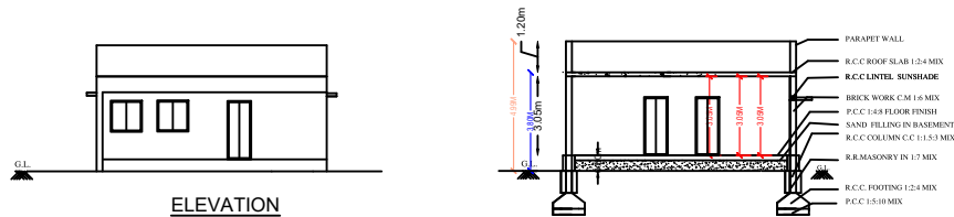
SECTION ON AB
