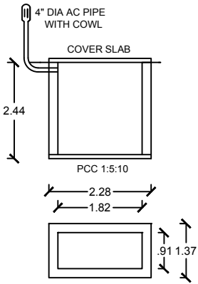
SEPTIC TANK
