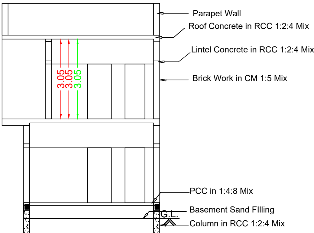
Section RR
