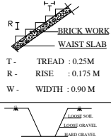
STAIRCASE DETAILS (NOT TO SCALE )
