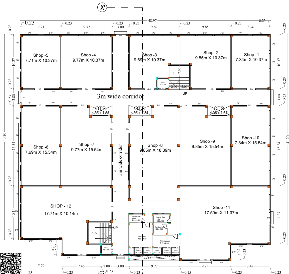
GROUND FLOOR PLAN (Mechanical Ventilator Provided)
