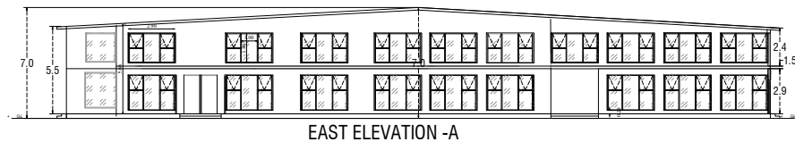
EAST ELEVATION - A
