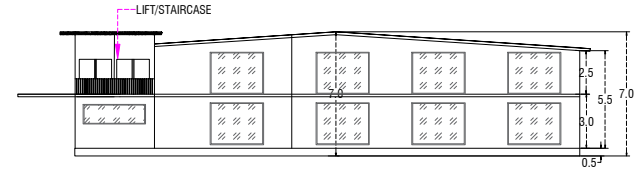
BLOCK -2 NORTHEAST ELEVATION
