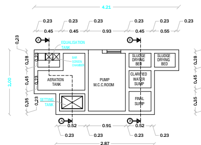
SEWAGE TREATMENT PLANT PLAN HYDRAULIC FLOW DIAGRAM SCALE: 1:100
