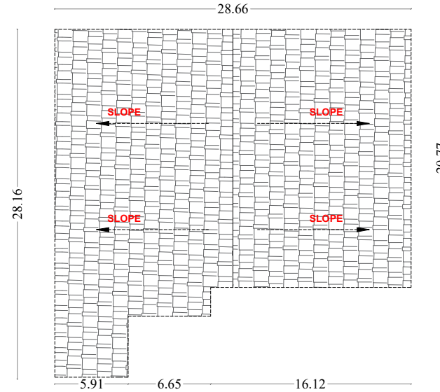
BLOCK -2 TERRACE FLOOR PLAN
