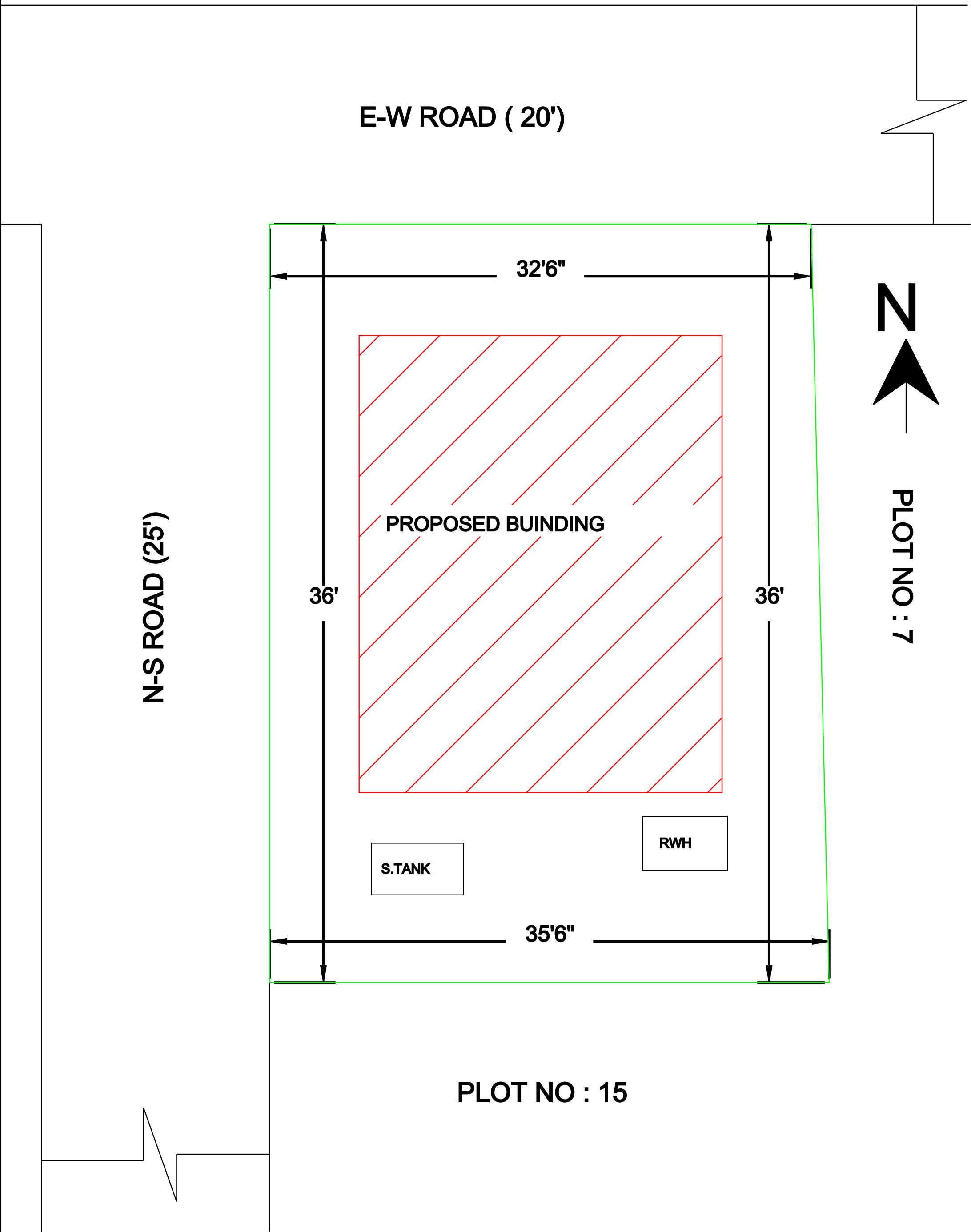
SITE PLAN
