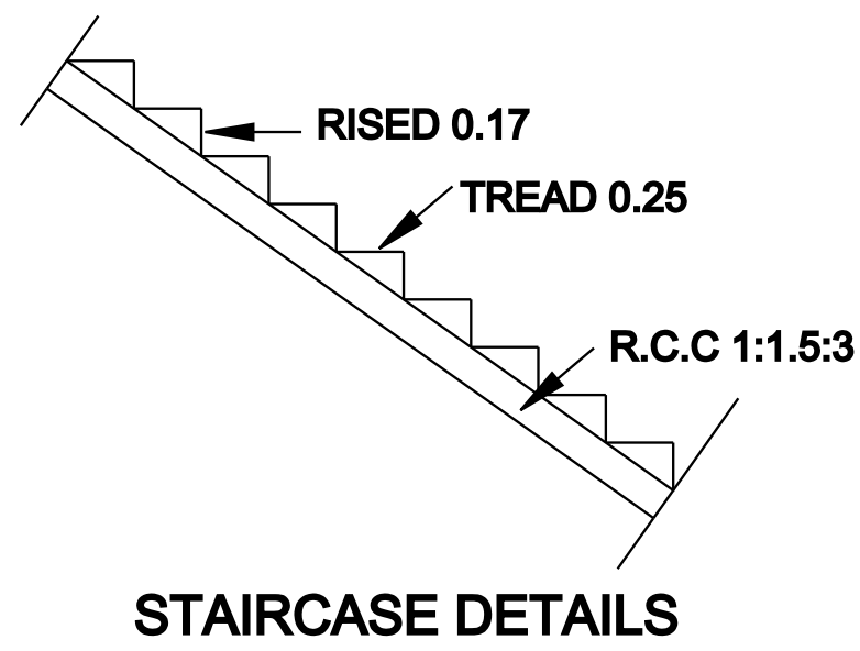
STAIRCASE DETAILS
