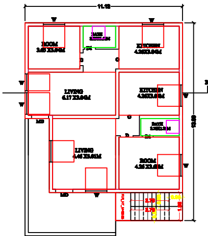
PROPOSED FIRST FLOOR
