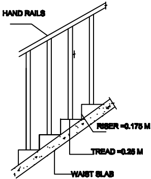
STAIR CASE DETAILS
