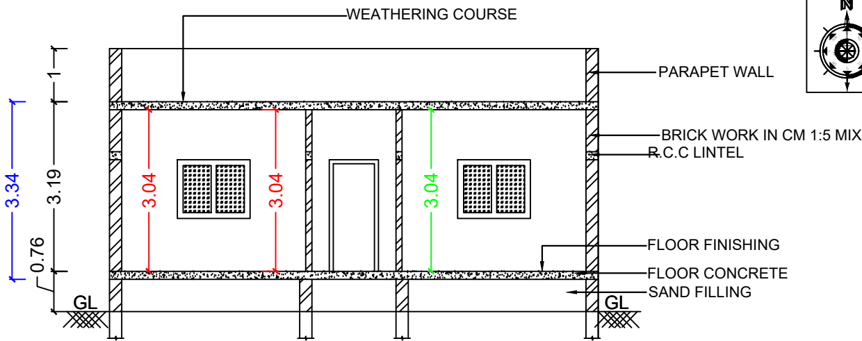
SECTION AT A1-A1
