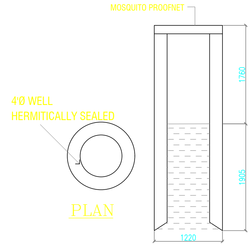
SECTION - BB DETAIL OF BORE WELL
