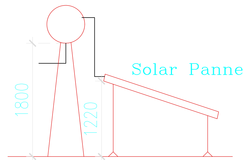
SIDE ELEVATION (Not to scale)
