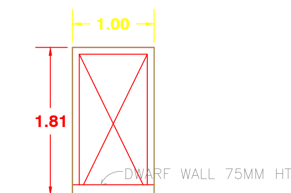
WIKET GATE ELEVATION
