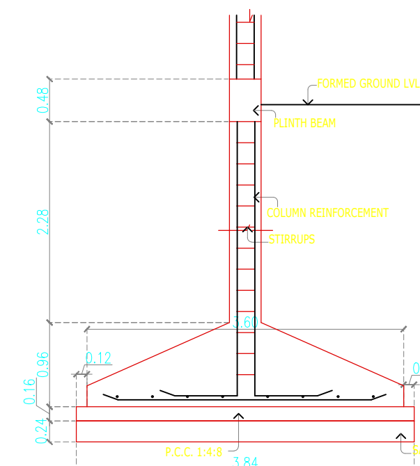
TYPICAL DETAIL OF COLUMN FOOTING
