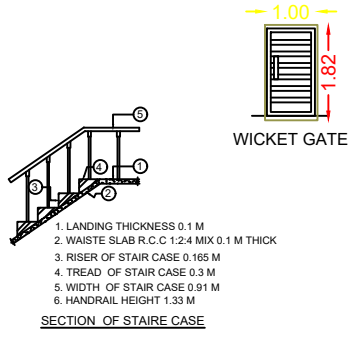
SECTION OF STAIR CASE
