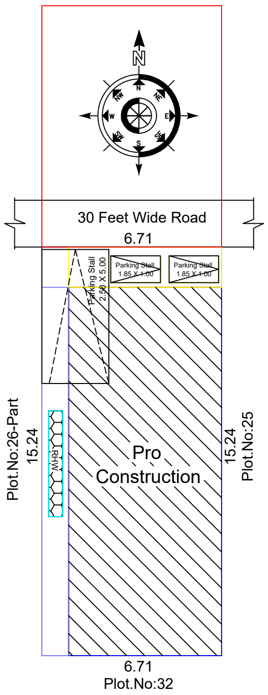
Site Plan
