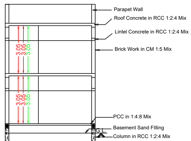
Section RR
