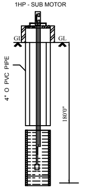
Bore Well Details
