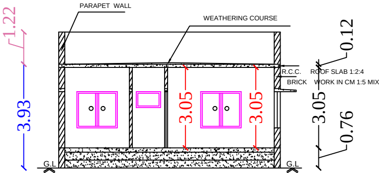
Section on-"AA"
