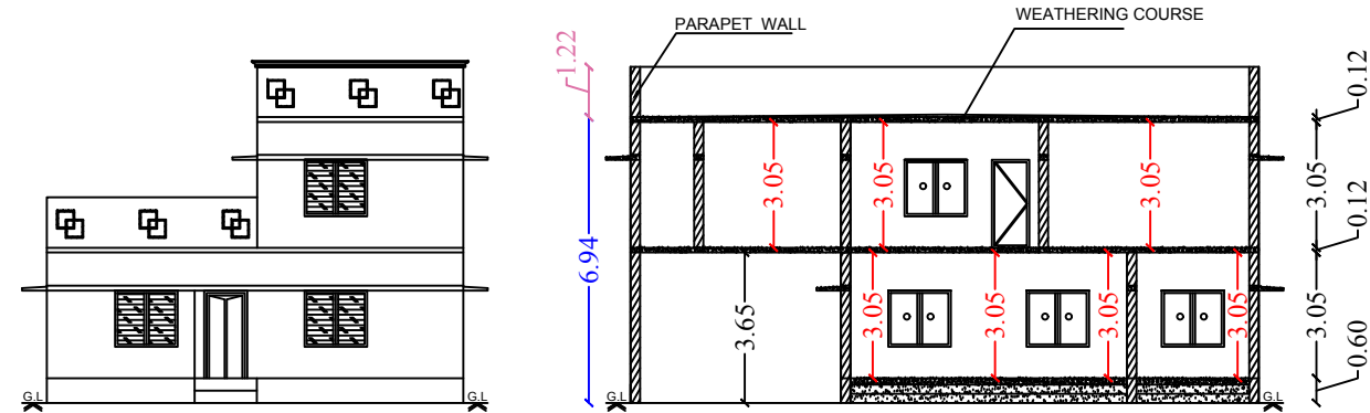
Front Elevation
