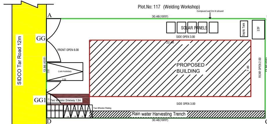
SITE PLAN 1: 100 SCALE
