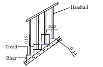
STAIRCASE DETAIL
