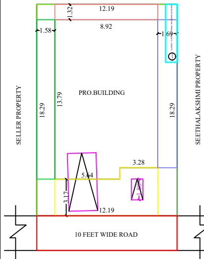
SITE PLAN
