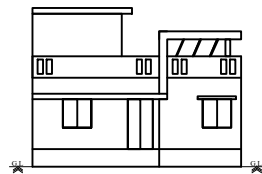
FRONT ELEVATION
