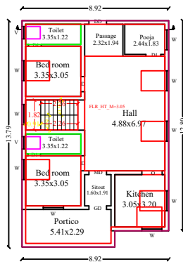
PRO.GROUND FLOOR PLAN
