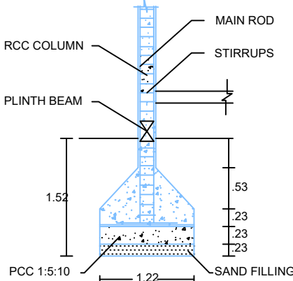
COLUMN DETAILS
