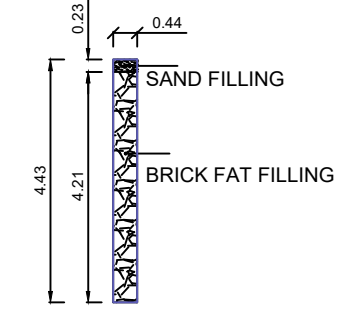
DETAILS OF PERCULATION PIT
