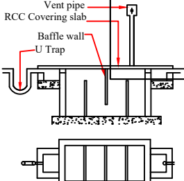
SEPTIC TANK
