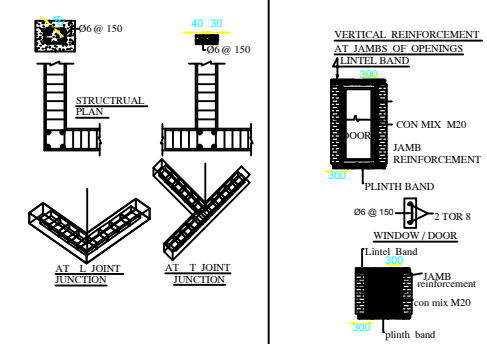
DETAILS OF EARTHQUAKE :
