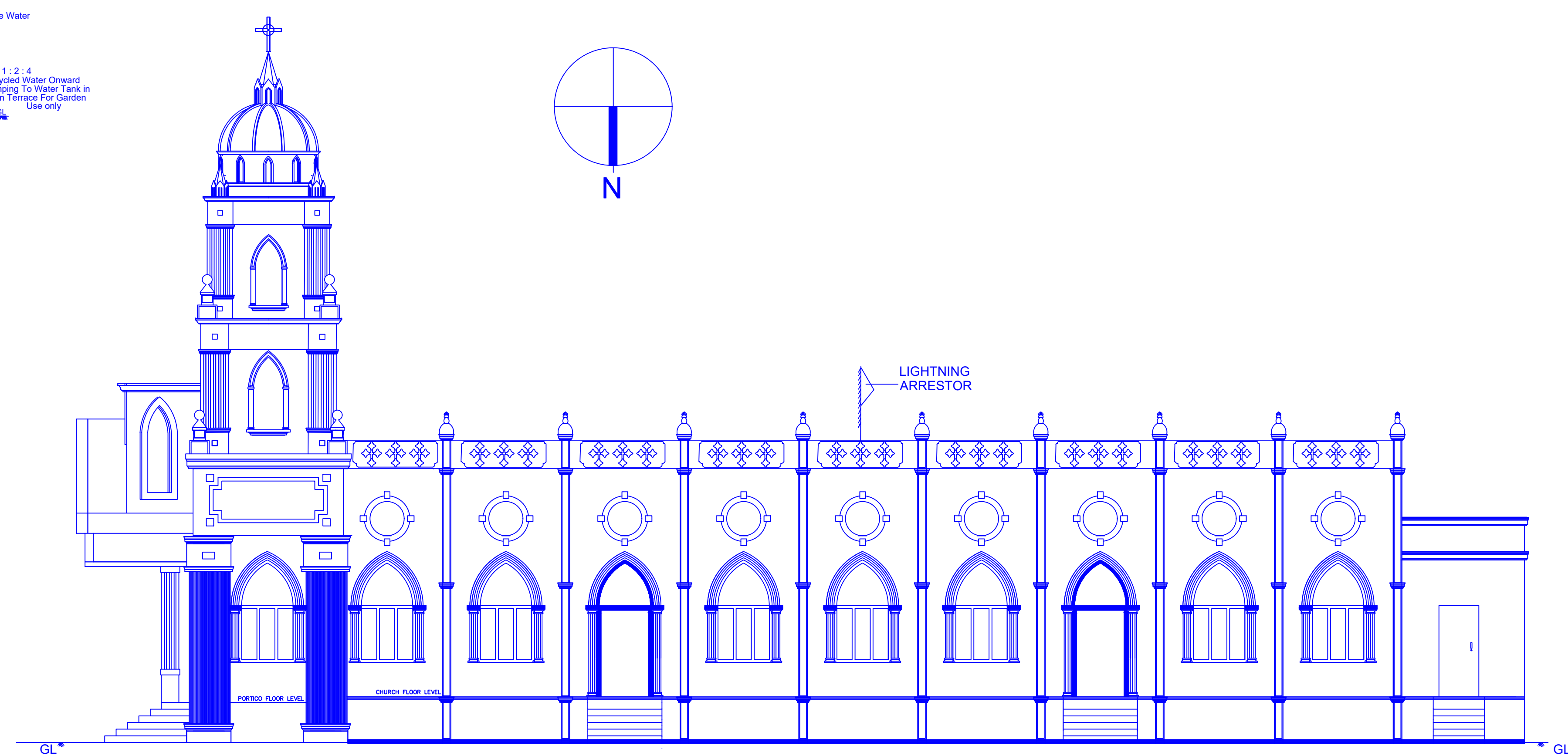
SIDE ELEVATION
