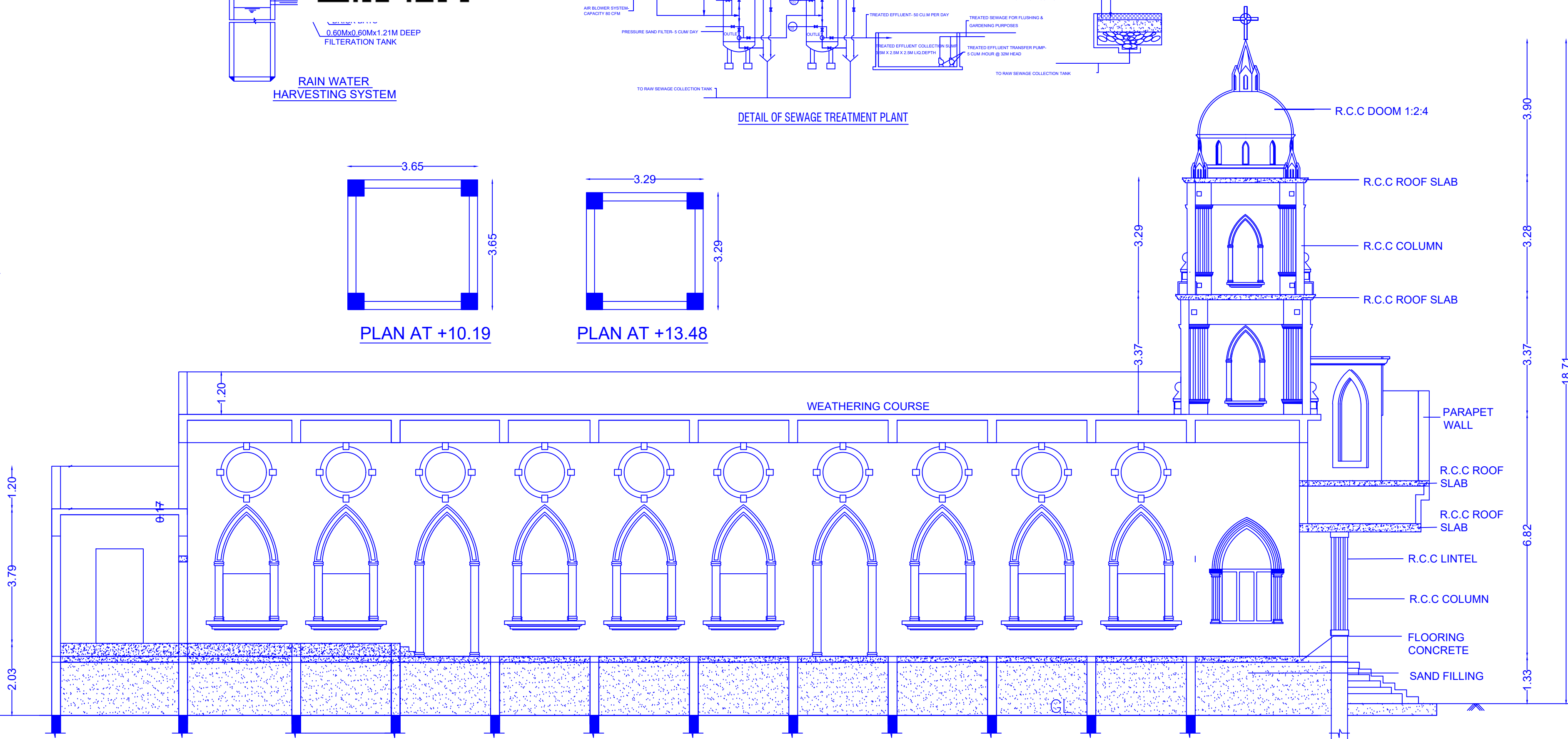
SECTION C-C
