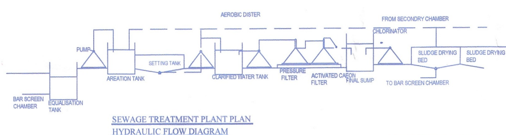
SEWAGE TREATMENT PLANT PLAN HYDRAULIC FLOW DIAGRAM
