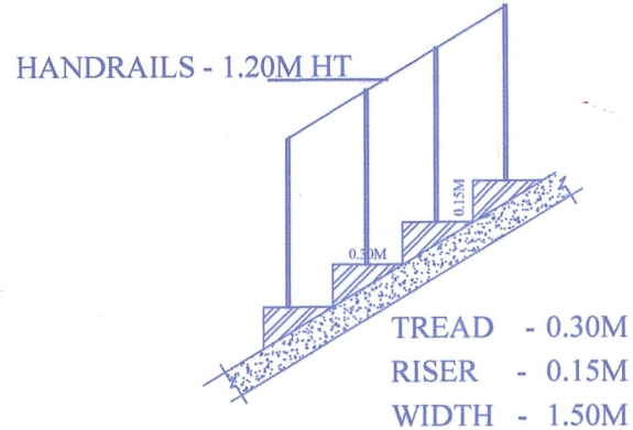
STAIRCASE DETAILS
