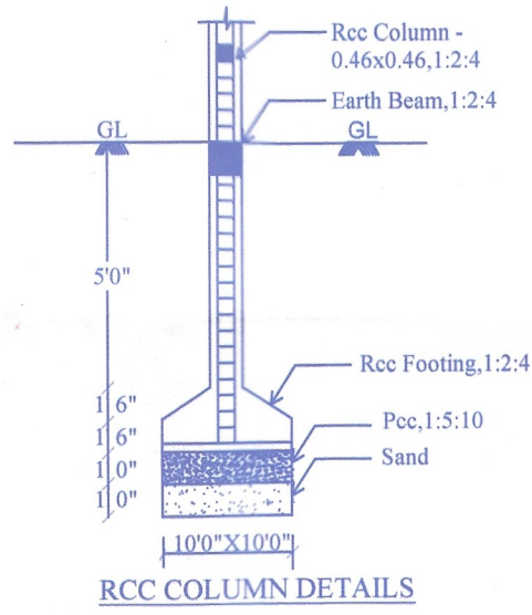
RCC COLUMN DETAILS
