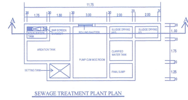
SEWAGE TREATMENT PLANT PLAN
