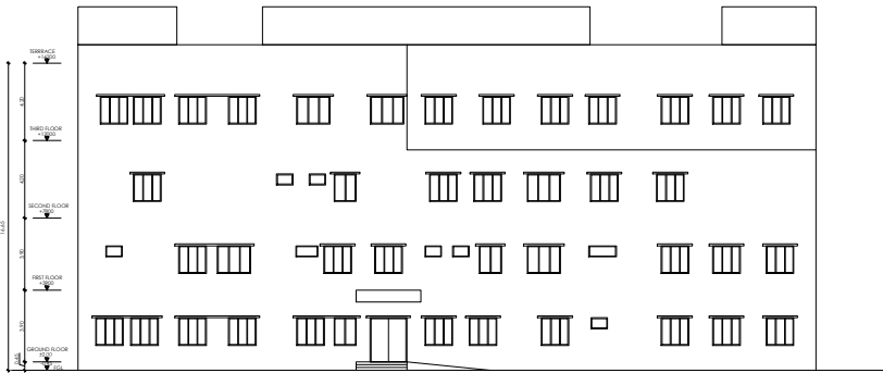
ELEVATION - B (BLOCK-1)
