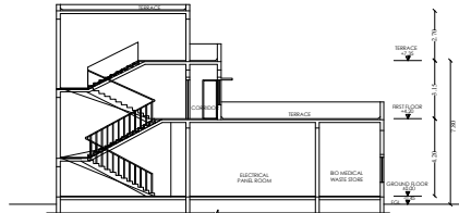
SECTION 2-2 (ADMIN BLOCK)
