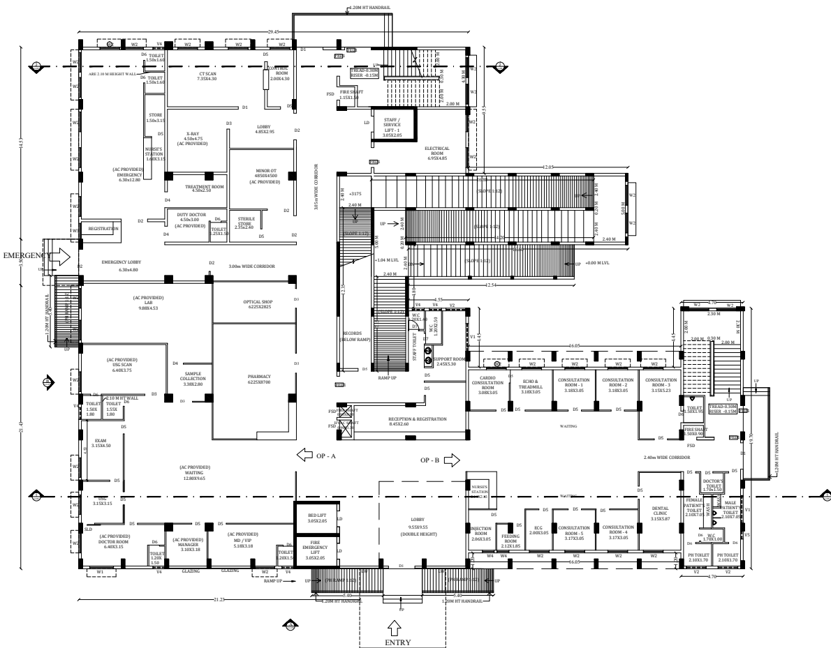
GROUND FLOOR PLAN (BLOCK-1)
