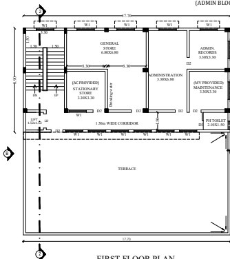
FIRST FLOOR PLAN (ADMIN BLOCK)
