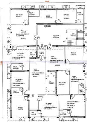
FIRST, SECOND AND THIRD FLOOR PLANS
