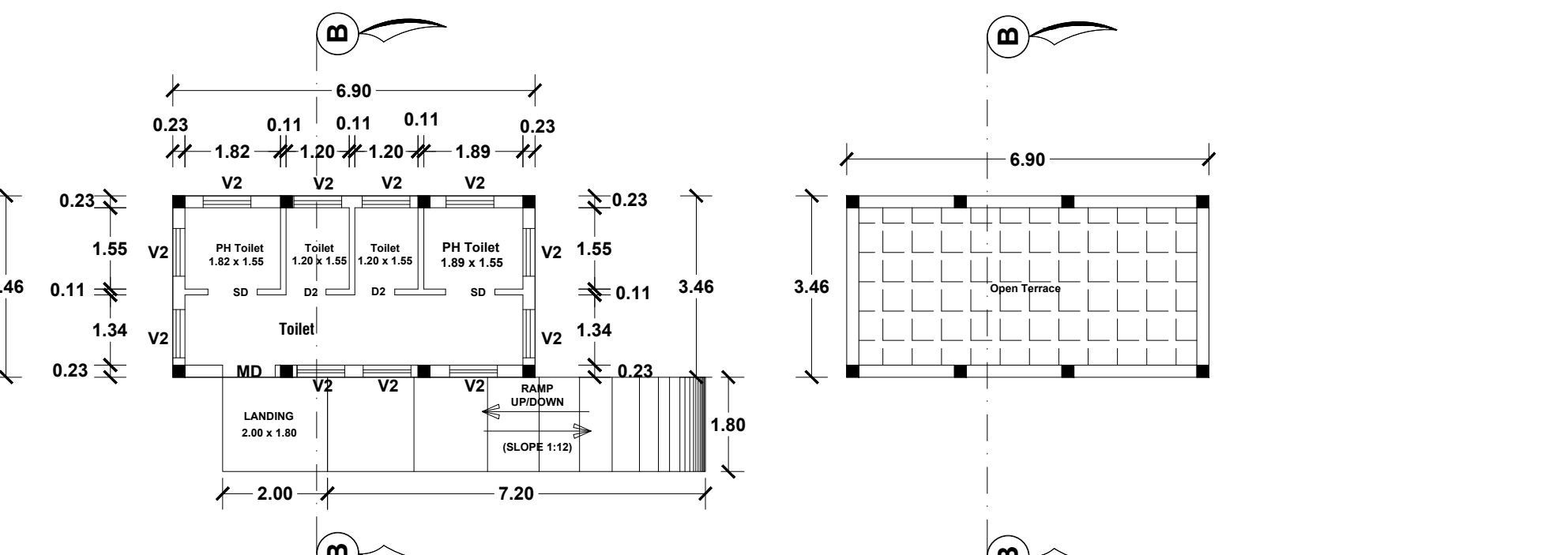
GROUND FLOOR PLAN BLOCK - 02 (Toilet Block)
