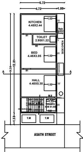
SITE PLAN CUM GROUND FLOOR PLAN
