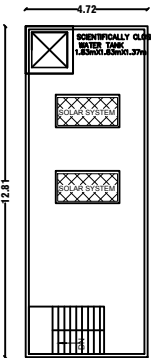
TERRACE FLOOR PLAN
