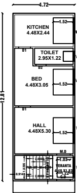
FIRST FLOOR PLAN
