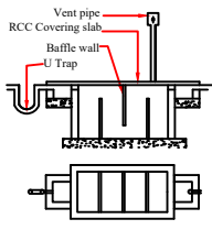
SEPTIC TANK
