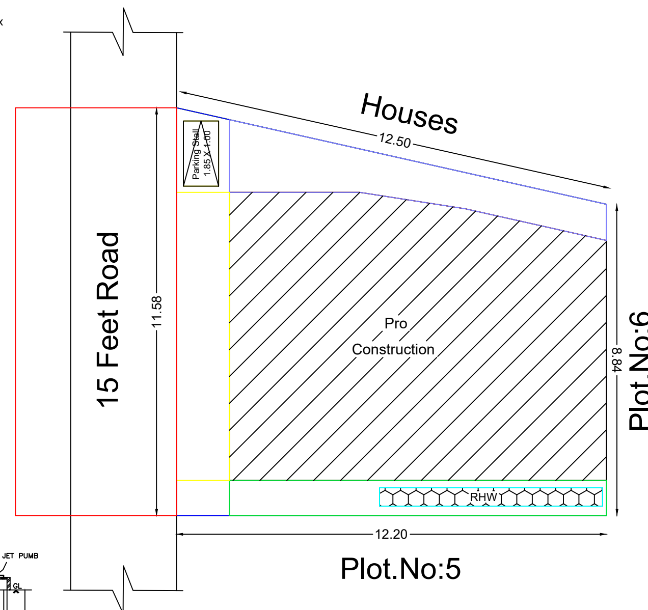
Site Plan
