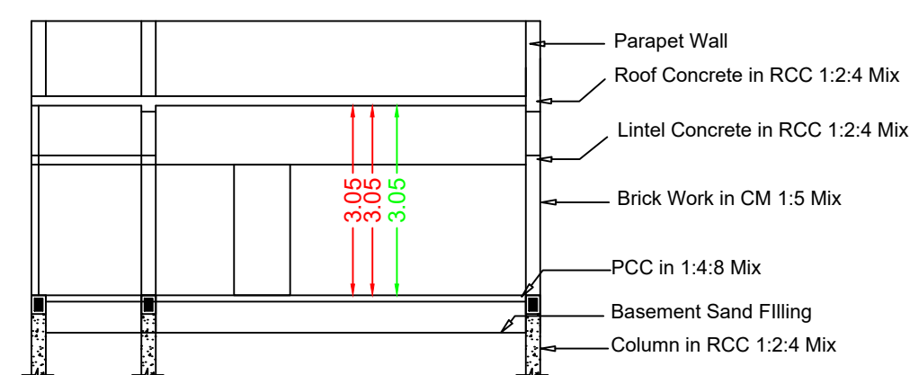
Section RR
