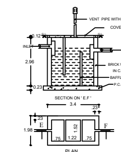
SEPTIC TANK DETAILS ( NOT TO SCALE )
