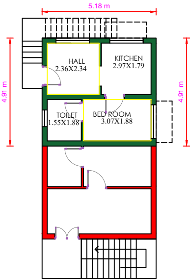
EXISTING AND PROPOSED FIRST FLOOR
