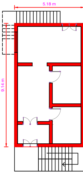
EXISTING GROUND FLOOR
