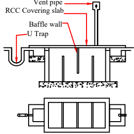
SEPTIC. TANK
