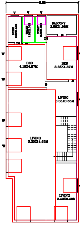
FIRST FLOOR
