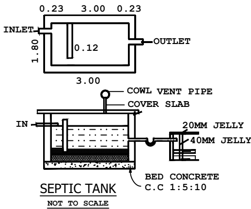
SEPTIC TANK NOT TO SCALE
