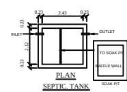
PLAN SEPTIC TANK
