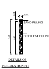
DETAILS OF PERCUSSION PIT
