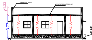
Section on-"AA"
