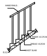
STAIR CASE DETAILS
