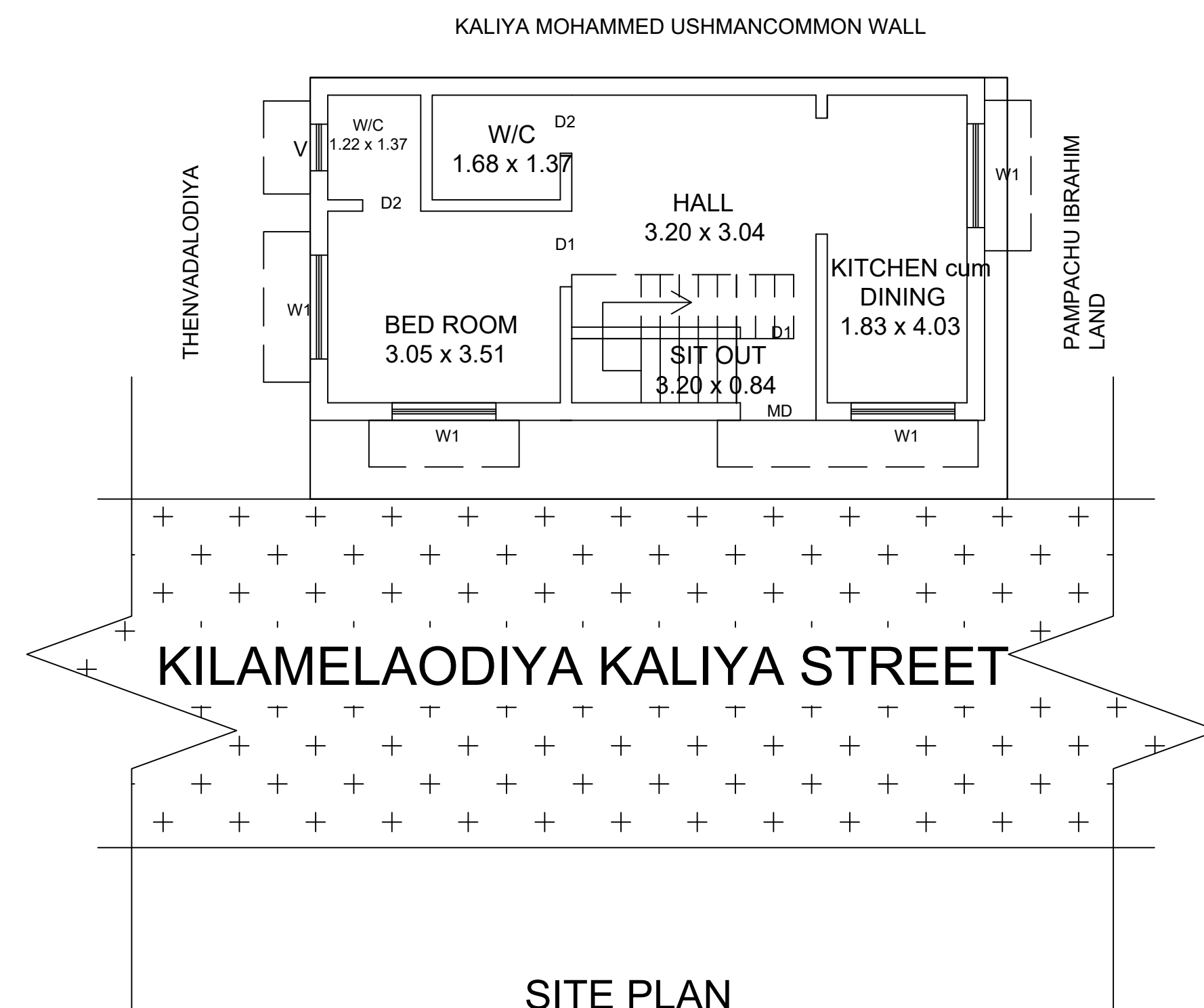
SITE PLAN
