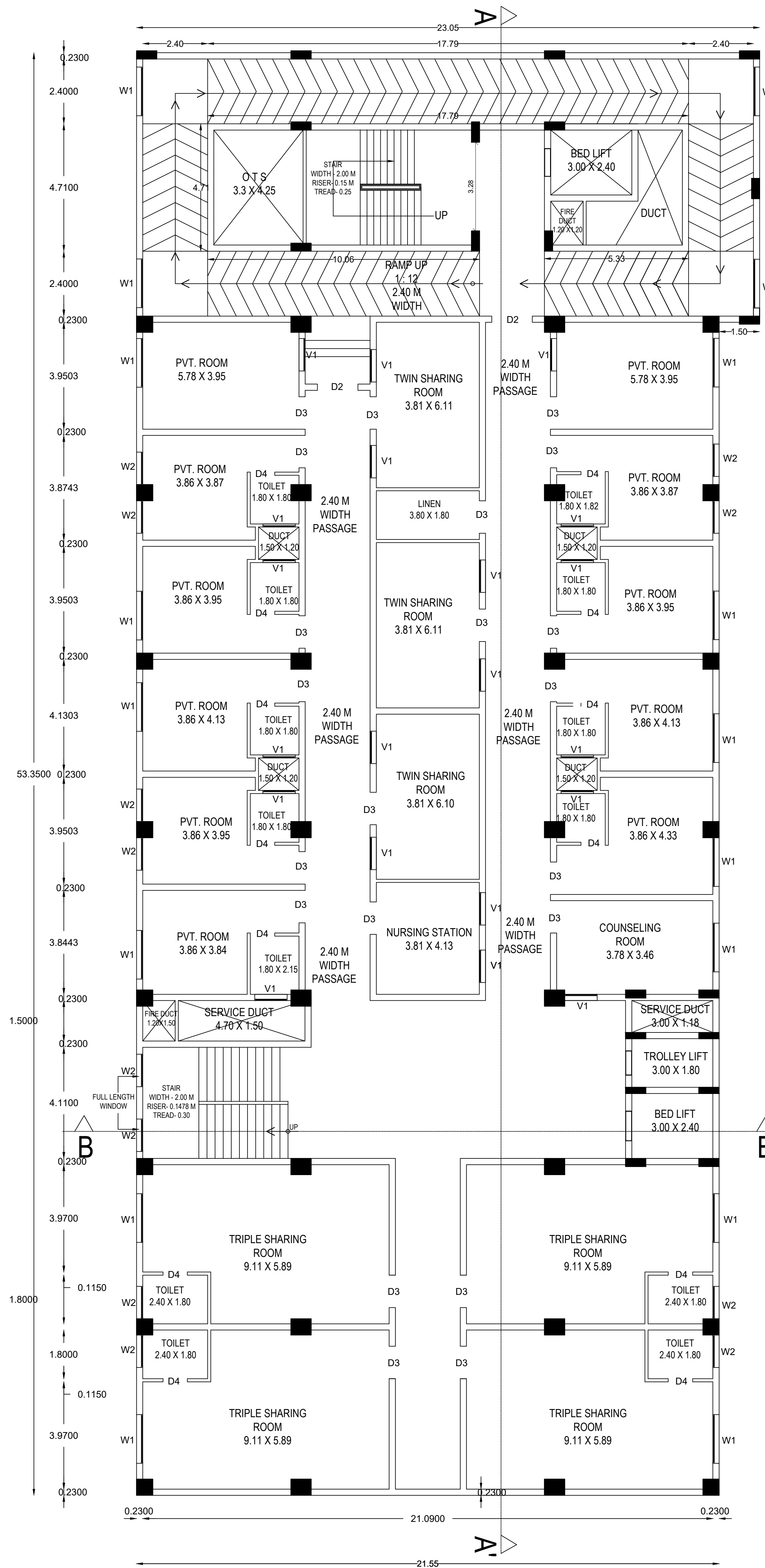
SIXTH FLOOR
