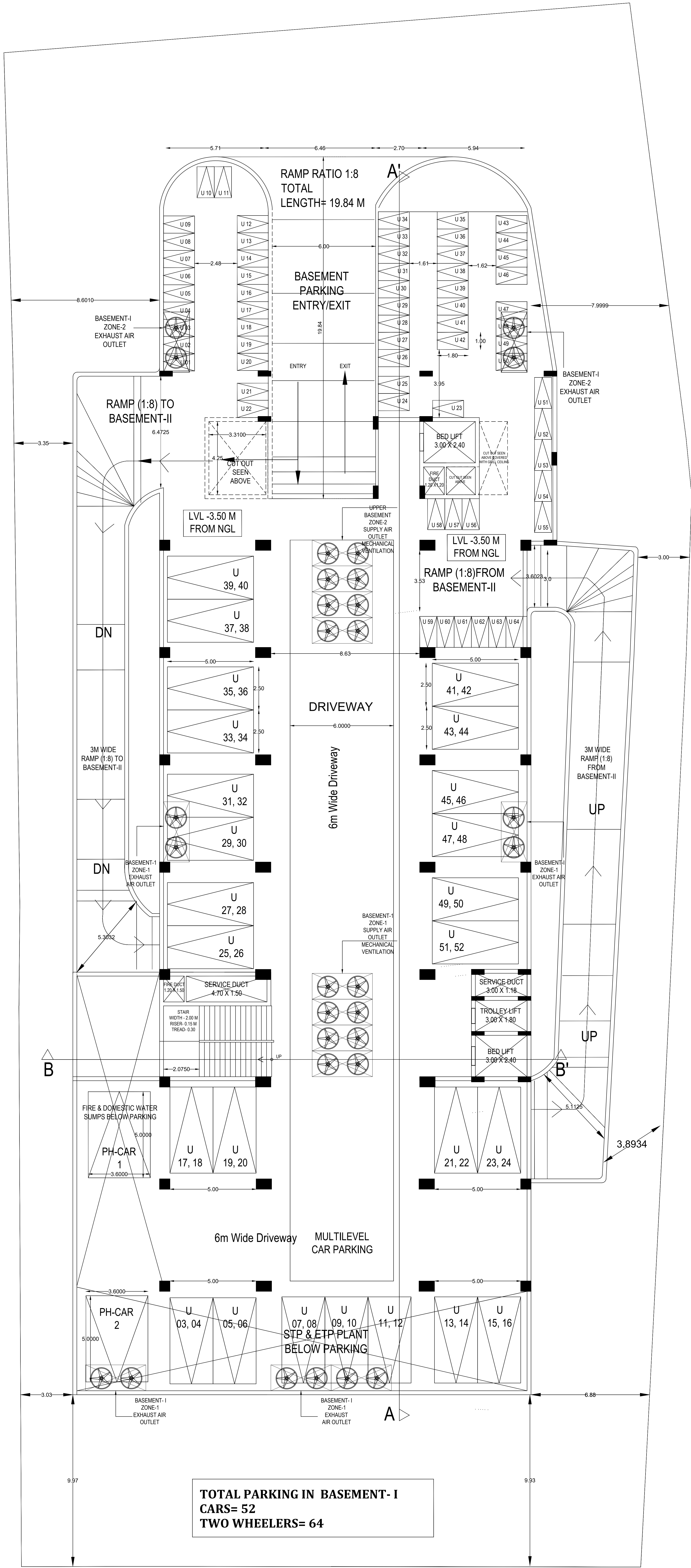
BASEMENT - I FLOOR PLAN
