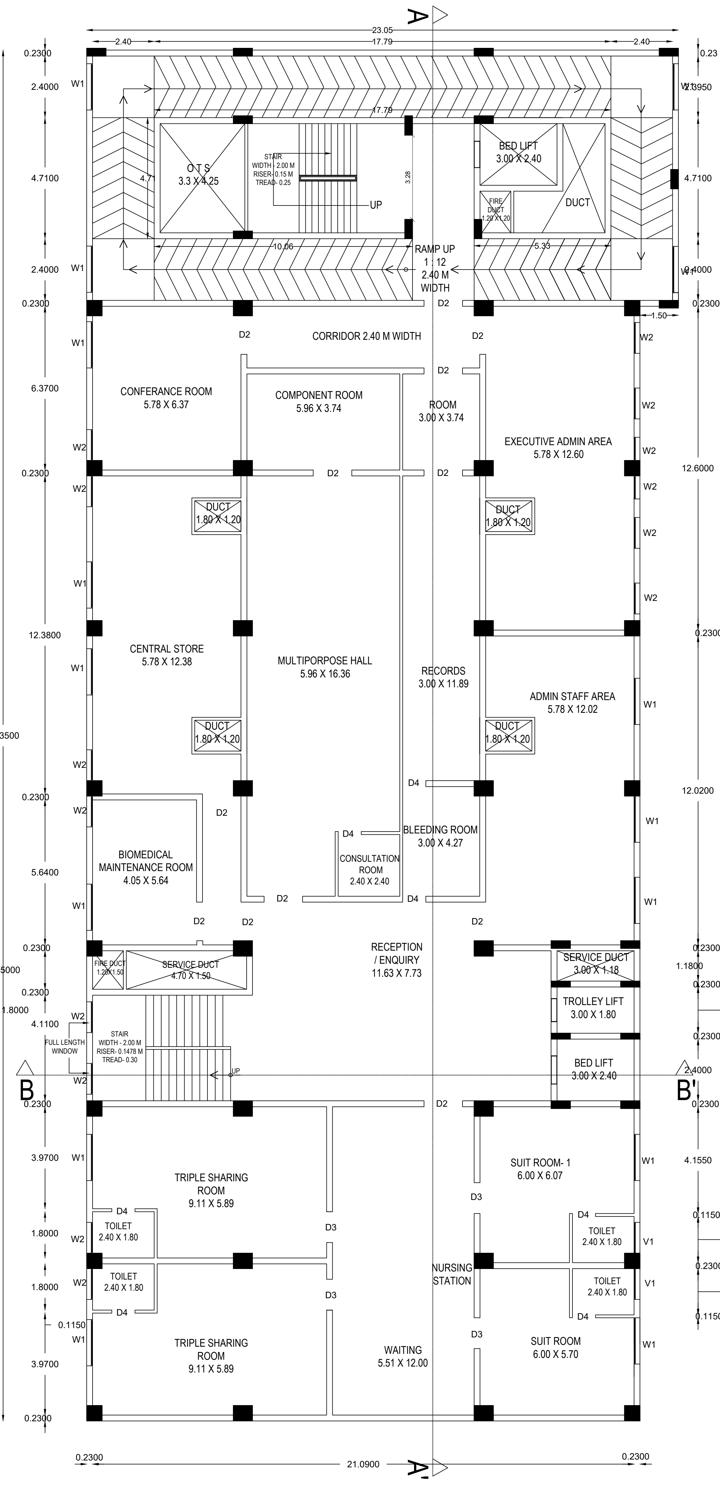
SEVENTH FLOOR
