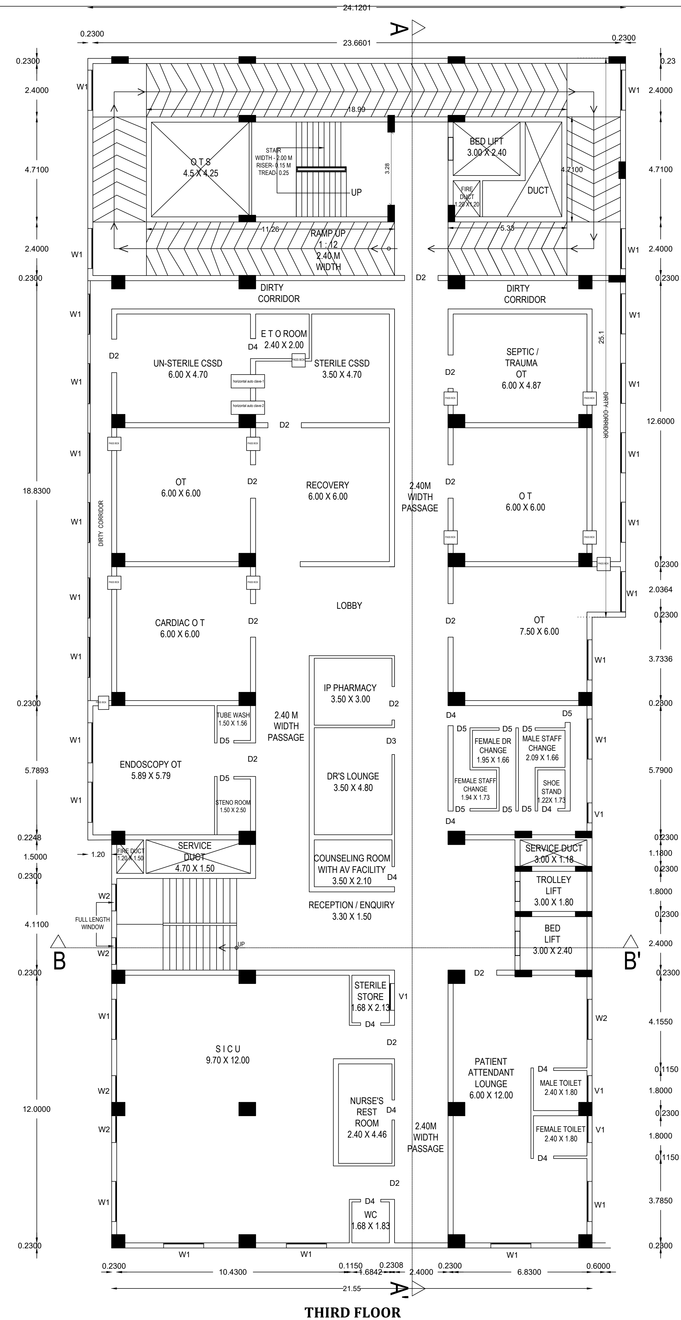
THIRD FLOOR
