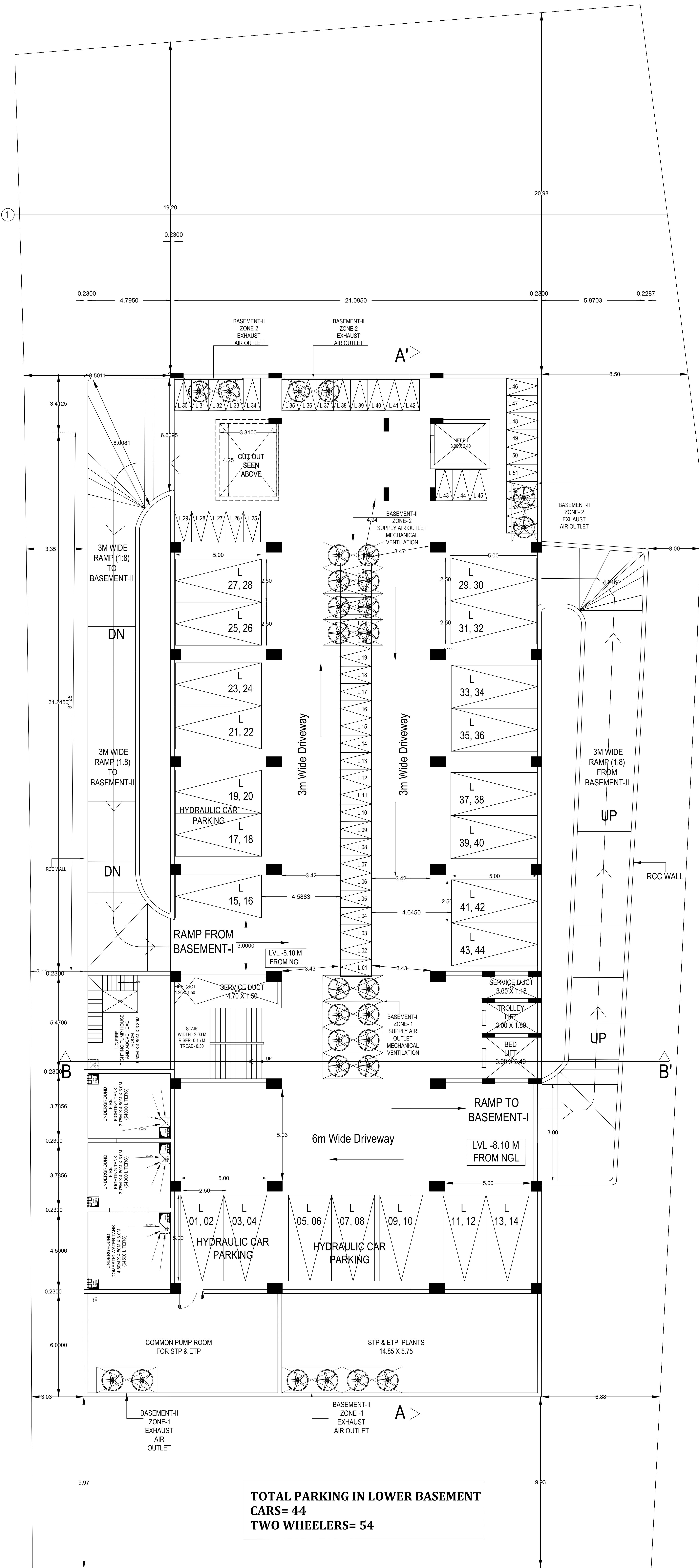
BASEMENT-II PLAN
