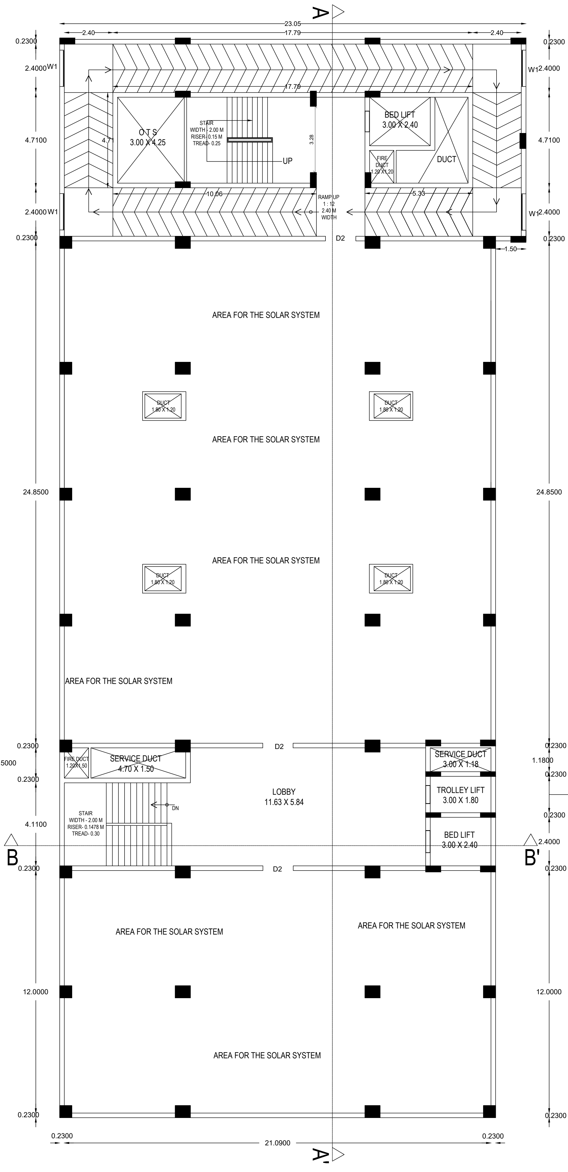
TERRACE FLOOR
