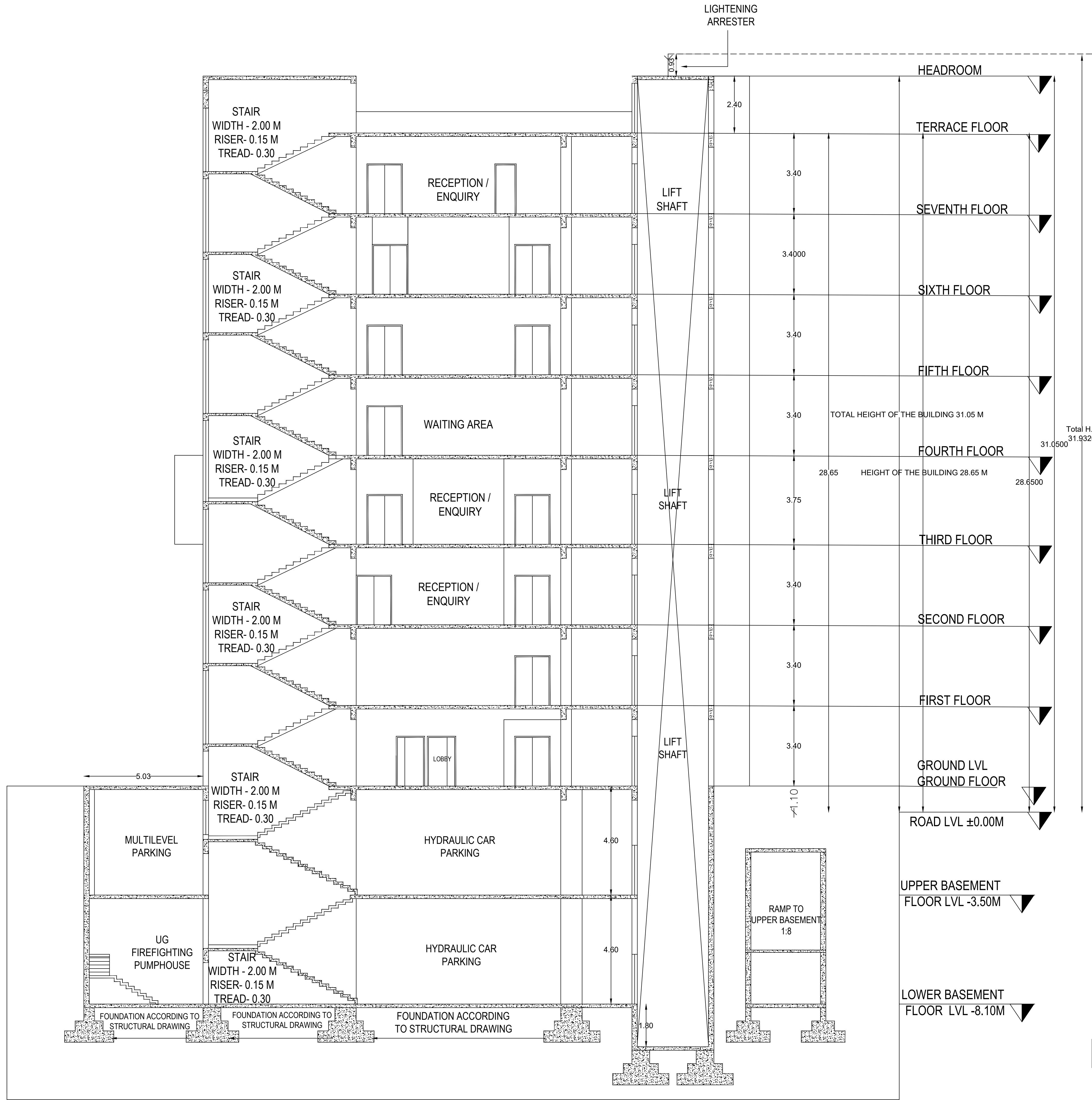
SECTION B-B'
