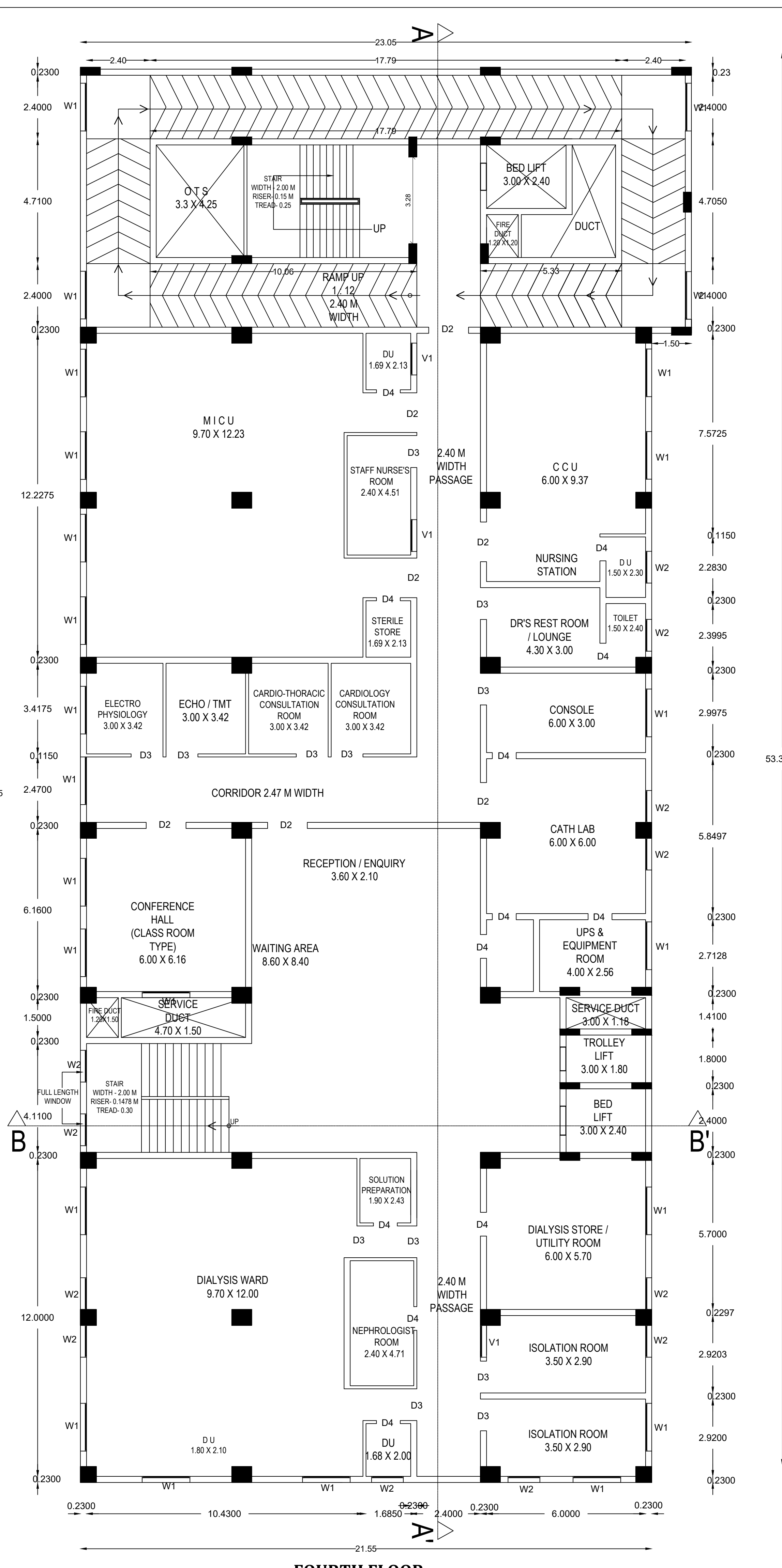
FOURTH FLOOR
