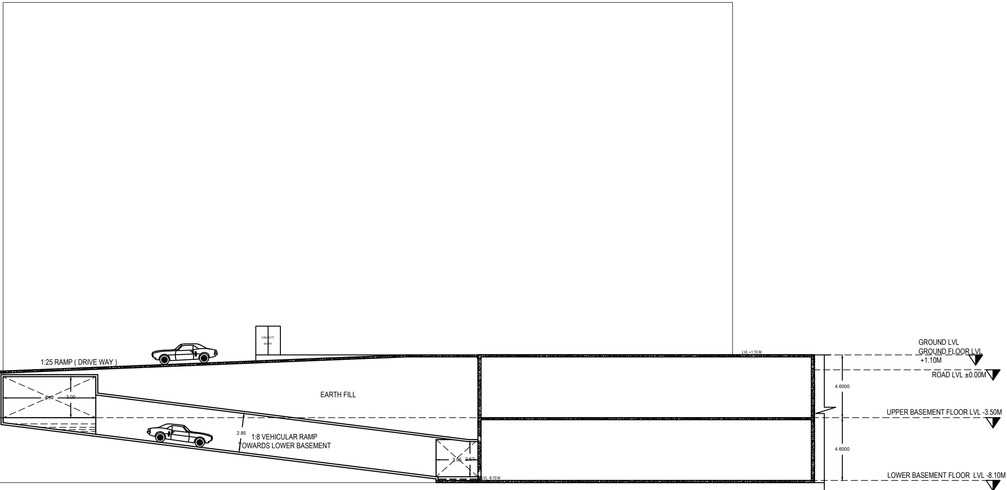
RAMP DETAIL
