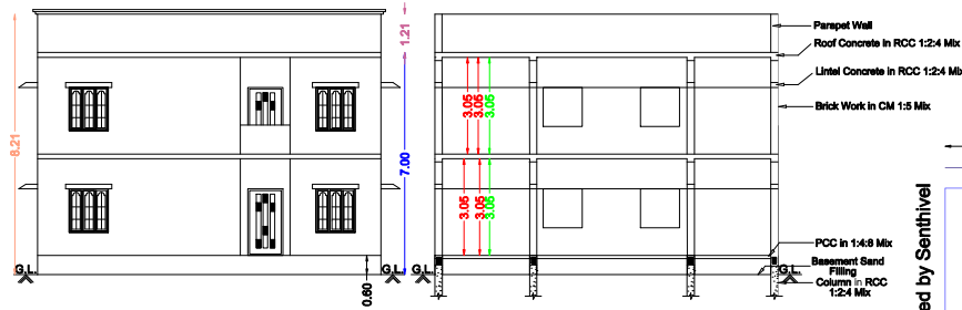
Front Elevation
