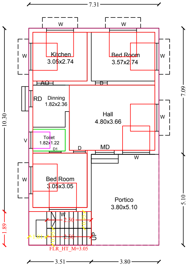
Floor - Ground
