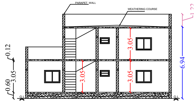
Section on-"AA"
