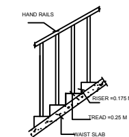
STAIR CASE DETAILS
