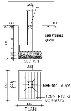
COLUMN & FOOTING DETAIL
