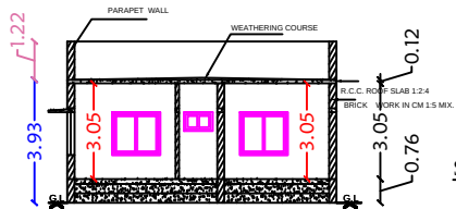
Section on-"AA"
