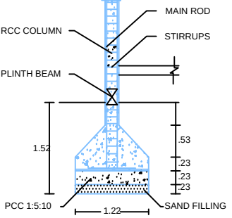
COLUMN DETAILS
