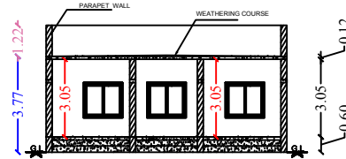
Section on-"AA"
