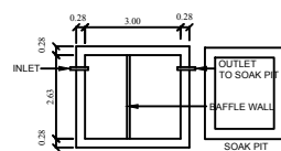
PLAN SEPTIC TANK
