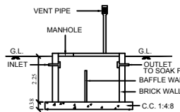
SECTION OF SEPT. TANK
