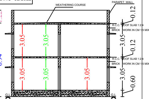
Section on-AA
