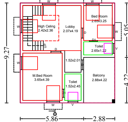
Floor - First
