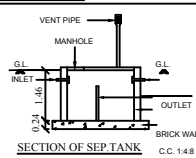
SECTION OF SEPTIC TANK
