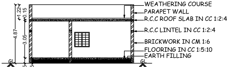
SECTION ON AB
