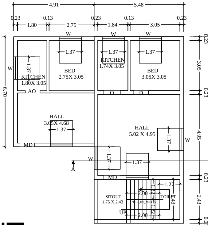
EX.GROUND FLOOR & ADDITIONAL PROPOSED CONSTRUCTION FOR GROUND FLOOR PLAN
