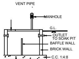
SECTION OF SEP. TANK
