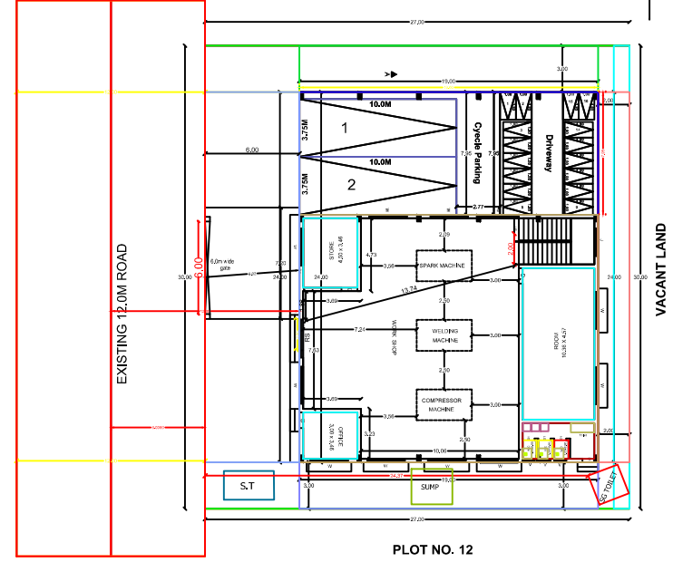
PLOT NO. 12 GROUND CUM SITE PLAN
