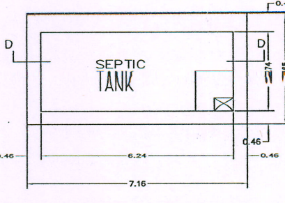
PLAN OF SEPTIC TANK SCALE 1"=2'0"
