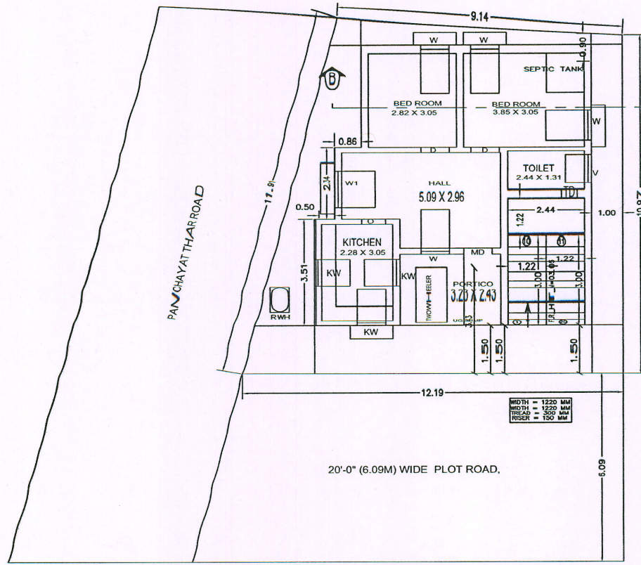
SITE CUM GROUND FLOOR PLAN
