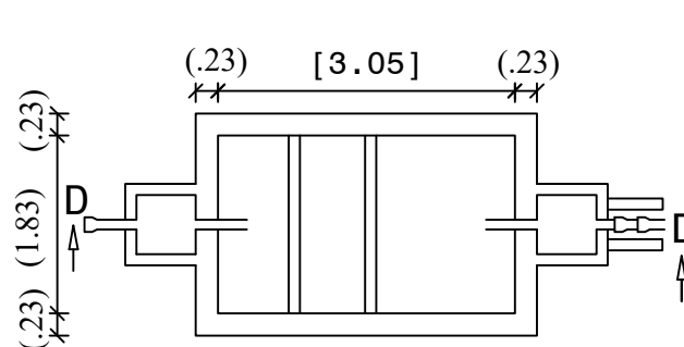
SEPTIC TANK PLAN
