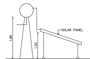
SIDE ELEVATION (NOT TO SCALE)
