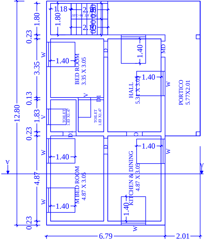
PLAN FOR GROUND FLOOR
