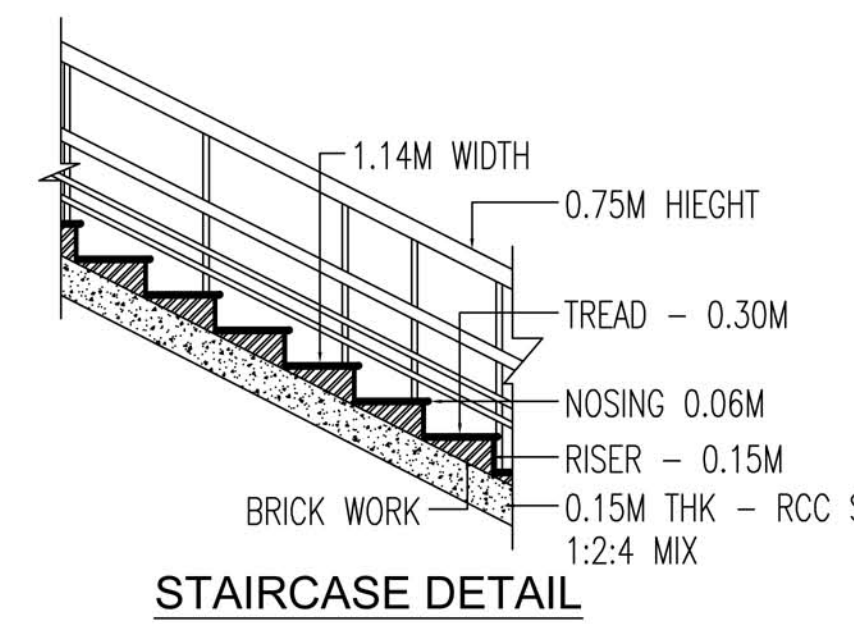
STAIRCASE DETAIL
