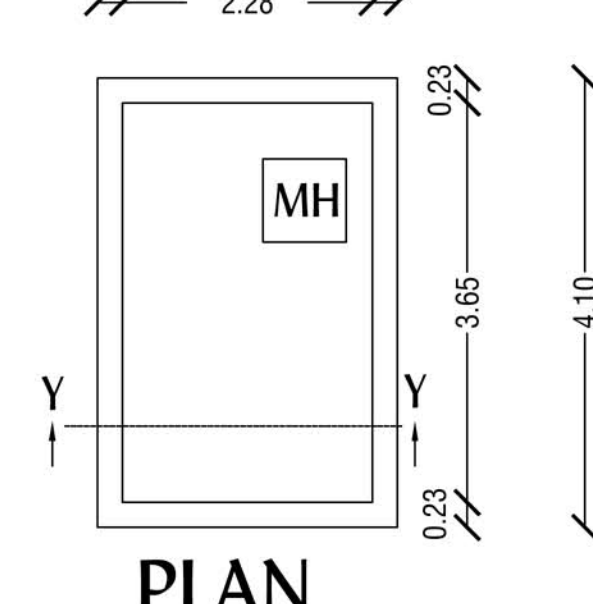
DETAILS OF U.G SUMP DRINKING WATER
