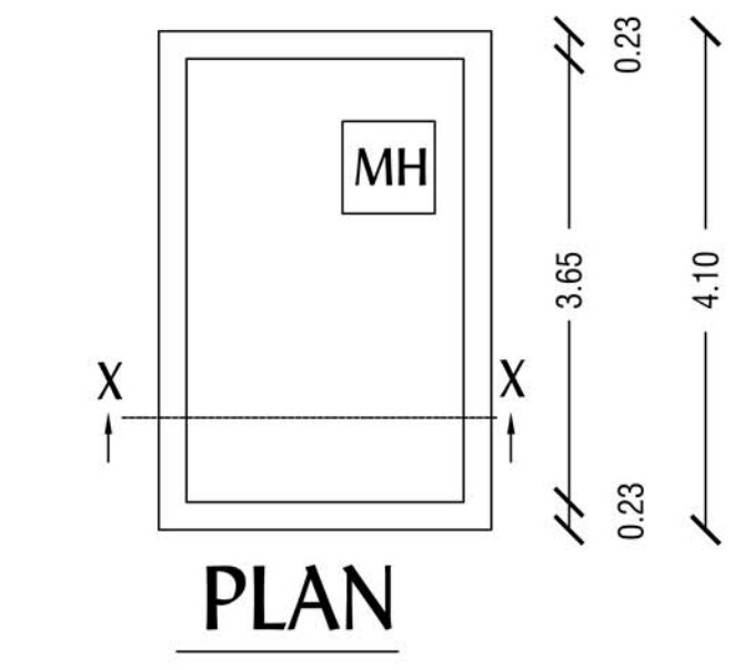
DETAILS OF U.G SUMP RAIN WATER COLLECTION SUMP
